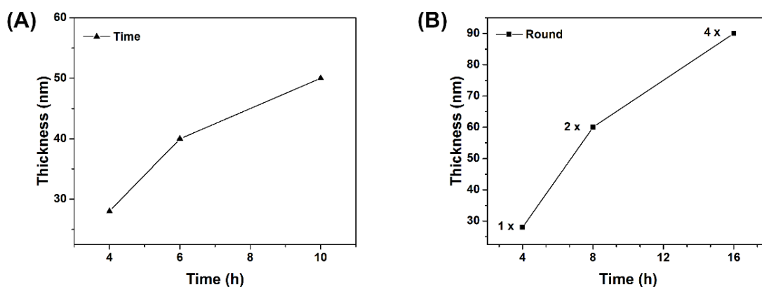
Figure A3 Dependence of the coating thickness on the coating time (A) and coating rounds (B).
