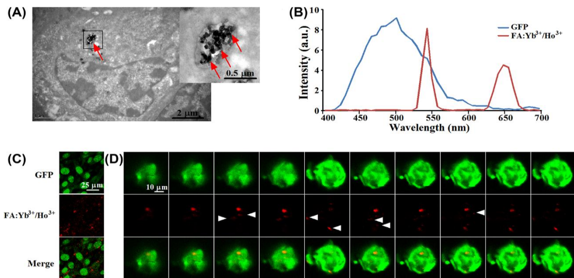
Figure 3-10 Uptake of FA:Yb 3+ /Ho 3+ crystals into BMSCs GFP . (A) TEM images of BMSCs GFP after incubation with 50 mg mL -1 FA:Yb 3+ /Ho 3+ crystals for 24 h at 37 °C. (Red arrows) (B) Fluorescence spectra of GFP and FA:Yb 3+ /Ho 3+ crystals. (C) Two-photon confocal luminescence images (excited by 980 nm light) of BMSCs GFP treated as in (A). (D) Two-photon confocal microscope scanning of BMSCs GFP after treatment with 50 mg mL -1 FA:Yb 3+ /Ho 3+ (excited by 980 nm light). (White triangle). Adapted with permission from Hu. [101] Copyright (2015) Elsevier.
