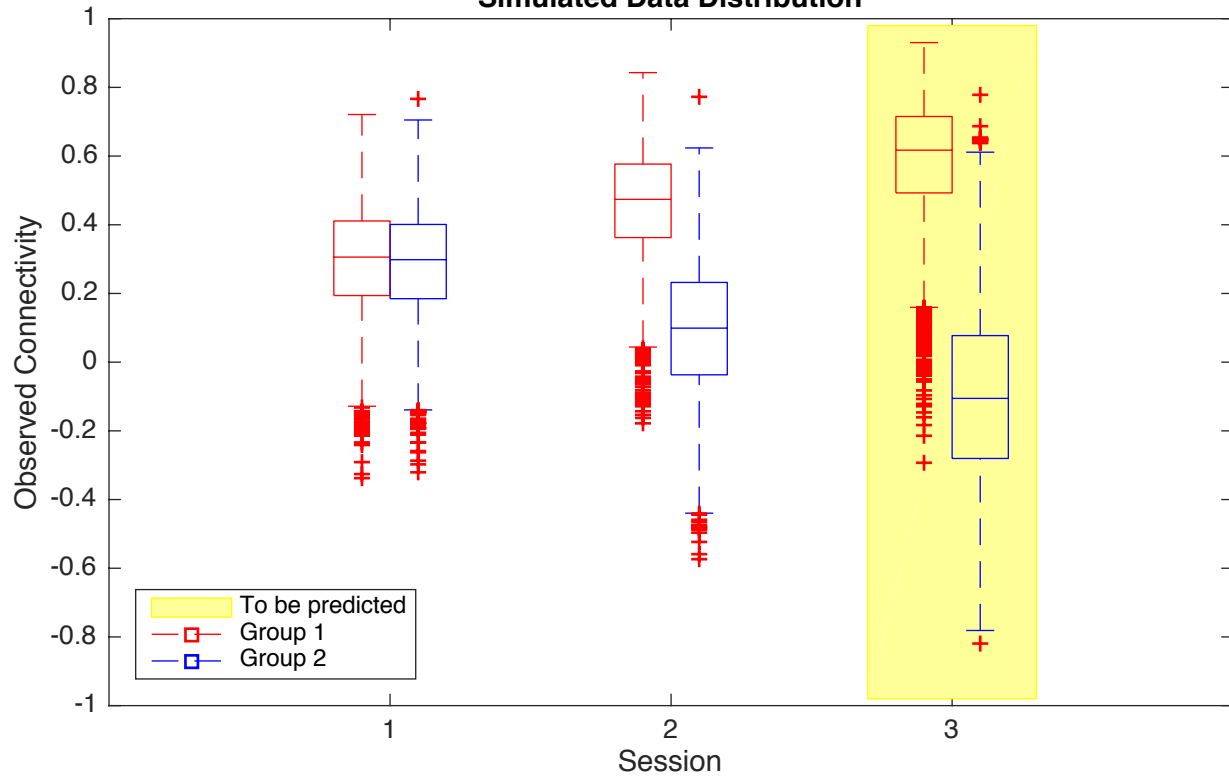
Simulated Data Distribution
