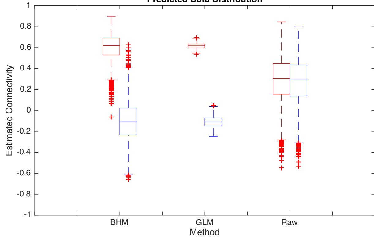
Predicted Data Distribution
