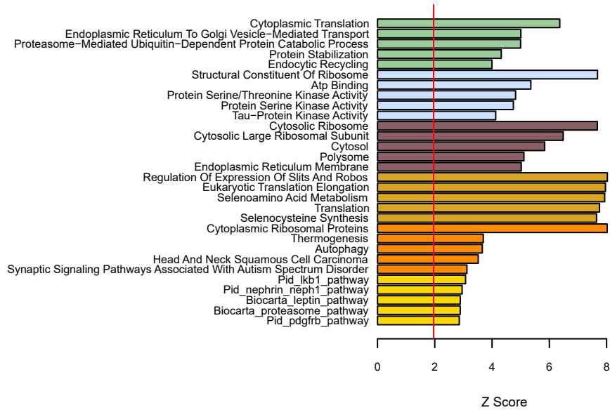
K-means Cluster 4
