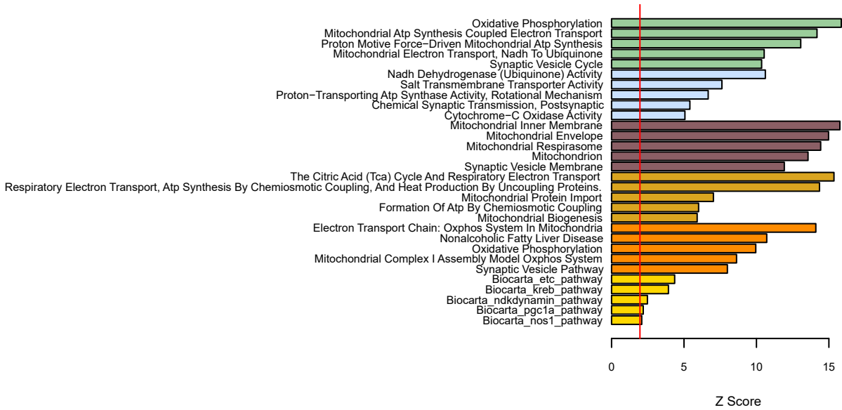
K-means Cluster 3
