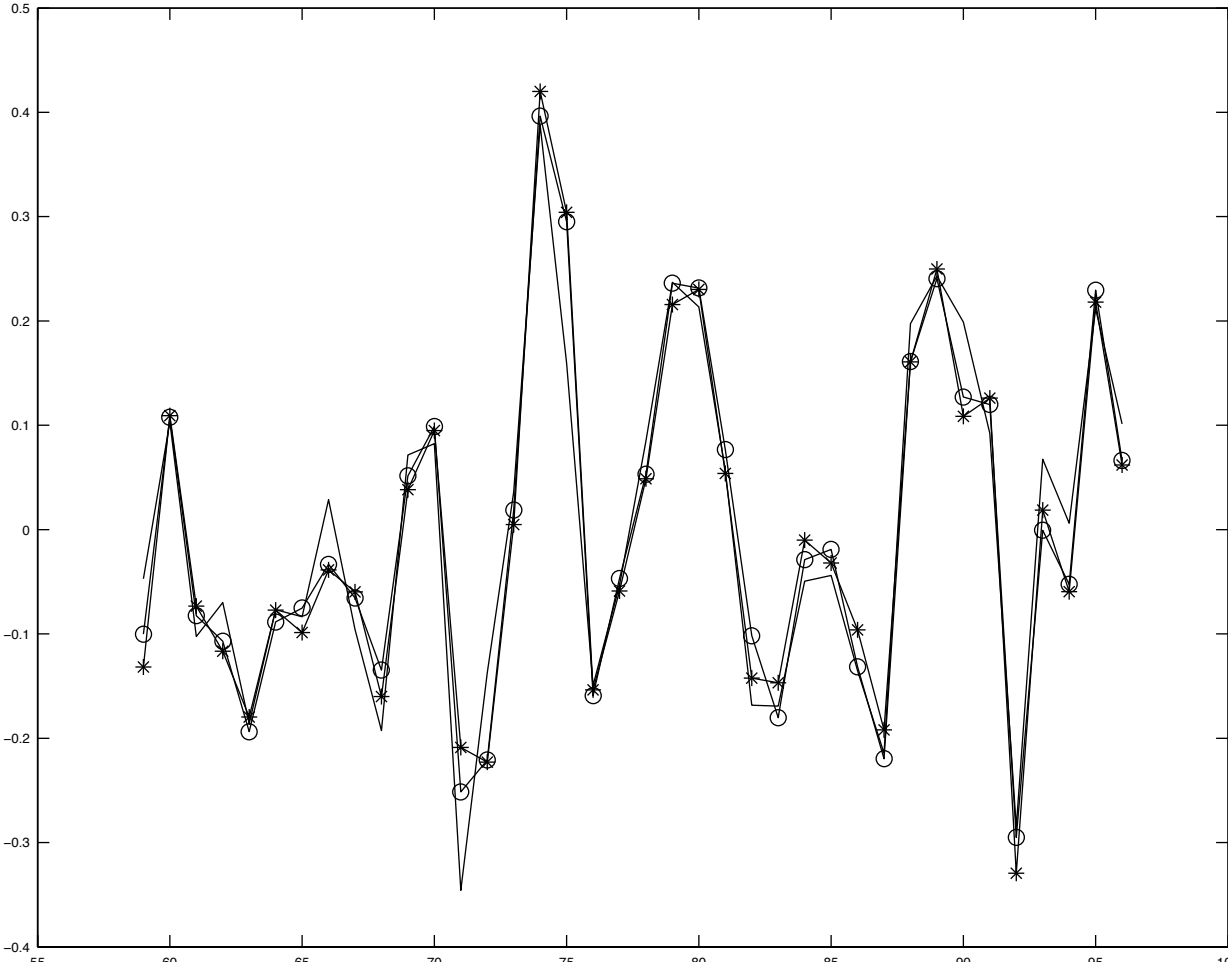
Graphs of Common Factors Extracted at Each Disaggregation Level:4-digit factor=stars; 3-digit factor=circles; 2-digit factor=solid red
