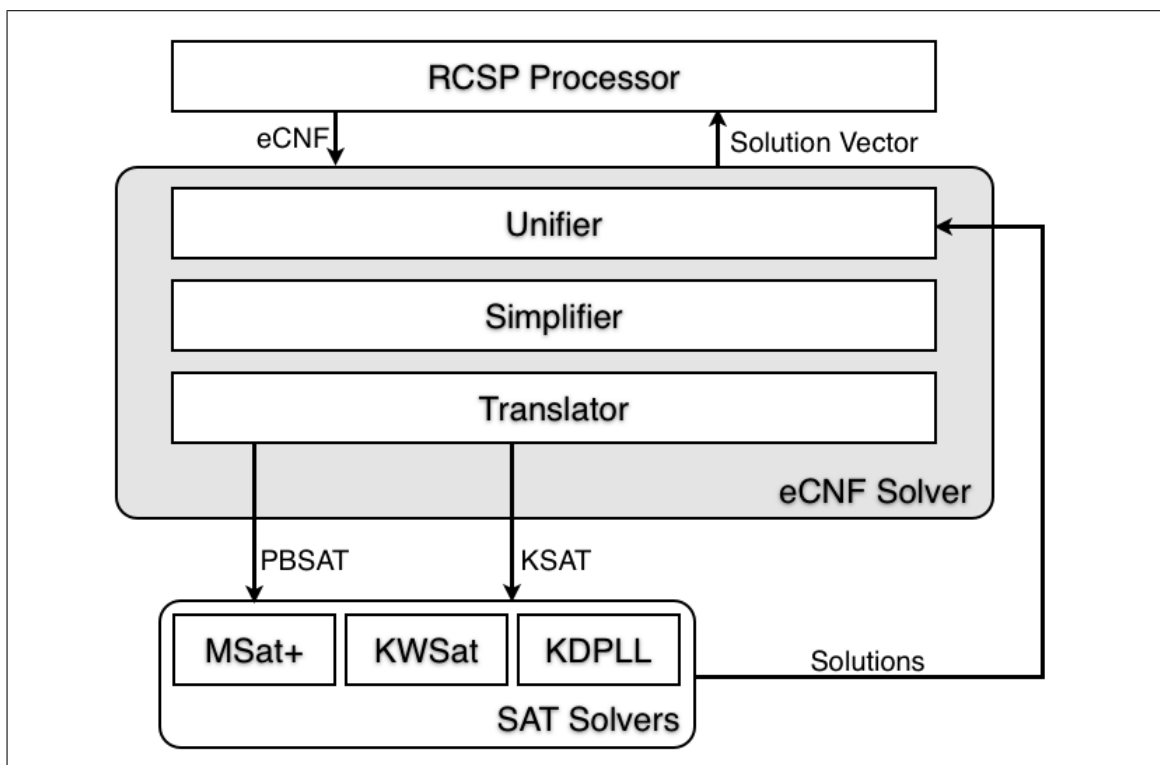
Figure 4.7: The eCNF Solver
