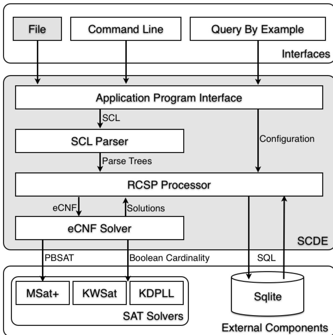
Figure 4.1: SCDE Architecture
